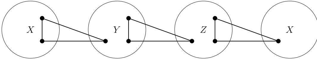
FIGURE 1. An extremal construction.
