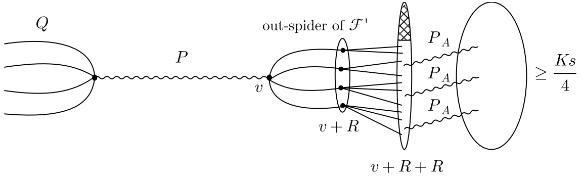
FIGURE 9. Illustration of the proof of Theorem 8.10. We take a maximal \mathcal{F} -absorbing fork (P, Q) whose final vertex is suitably extendable. The everywhere-expansion of the set E provides many potential ways to extend P by following a leg of the out-spider, then taking one more step using a colour from a different gadget, and finally appending a translate of a short rainbow path P_A . The maximality hypothesis ensures that in fact P already used nearly all of the colours of S , and we can integrate the remaining colours using one of the legs of Q .
