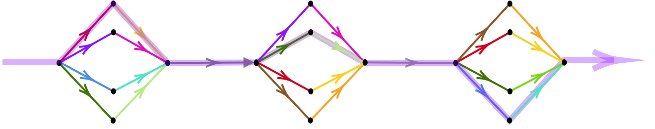
FIGURE 10. A waveform with three theta-graphs. Notice that some colour pairs repeat across the theta-graphs. A rainbow path omitting the brown-orange colour pair is highlighted.
