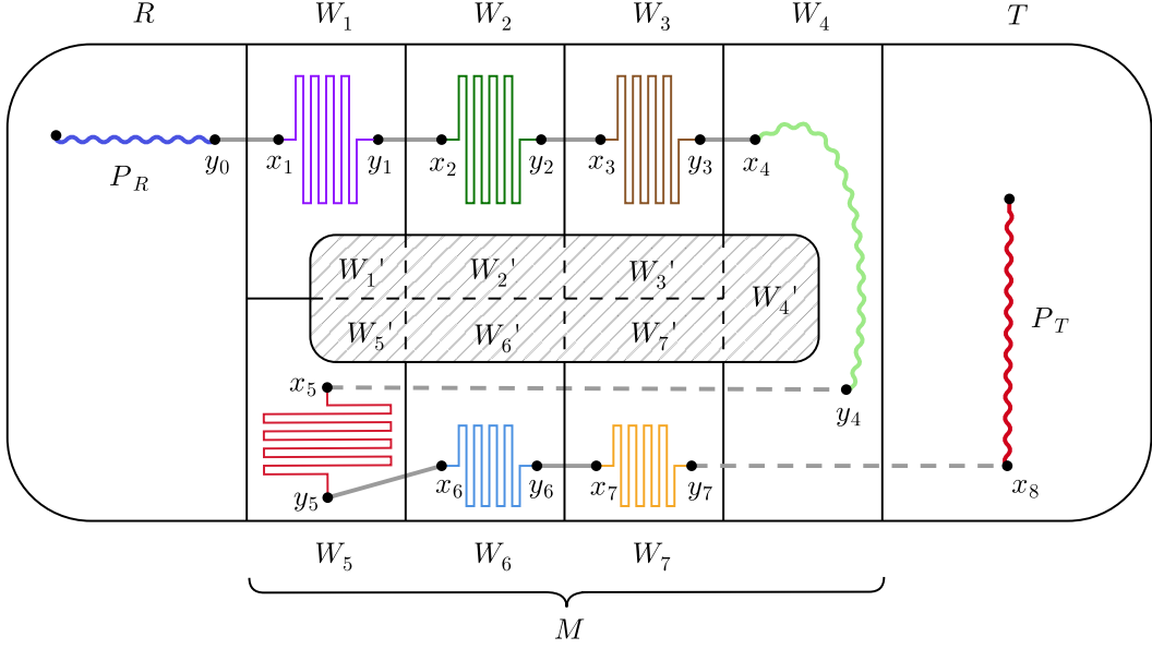
FIGURE 8. Illustration of the argument in Theorem 8.7 with t = 4, m = 3 . W_1, W_5; W_2, W_6; W_3, W_7 are pairs of cosets of the same subspace, and the W_i 's are chosen to have very small intersections W'_i with the other W_j 's. We also have fixed “connection points” y_0, x_1, y_1, \dots, x_7, y_7, x_8 . P_R is an absorbing path built inside a random subset R . Each P_{M,i} is a rainbow path from x_i to y_i built in the intersection of W_i with a random set M , while avoiding W'_i and all of the other connection points. The path P_T uses up all of the unused colours, with the help of some gadgets activated in P_R .
