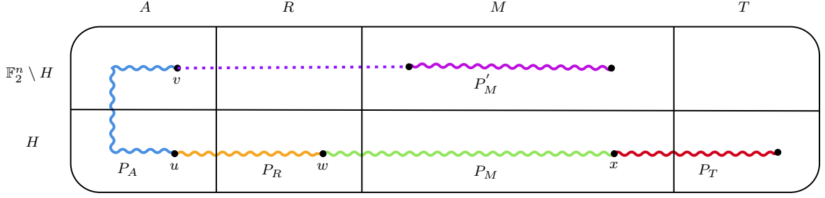
FIGURE 7. Illustration of the rainbow path constructed in the proof of Theorem 7.3. The dashed line indicates that the path P'_M does not intersect R . Colours indicate the different segments of the path, which of course are all rainbow with disjoint colour sets (except for P_T and P_R , whose colours are disjoint only after we activate the appropriate gadgets to replace P_R by P'_R ). The picture depicts the case \sum J \notin H ; the other case looks only marginally different ( P_T might “jump” once from T \cap H to T \setminus H at the point where it uses an edge of the colour that we removed from P_A ). P_A uses the colours J \cup S'_F ; P'_M uses the colours S_1 \cup S''_F , P_R uses the colours S_F ; P_M uses the colours S_0 \setminus (S_F \cup S'_F \cup S''_F \cup L) ; and P_T uses all but at most one of the colours of L \cup \bigcup_{F \in \mathcal{F}'} F .
